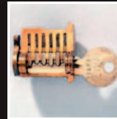
Original Yale pin tumbler
